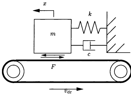
Fig. 5. 1-DOF model with dry friction
