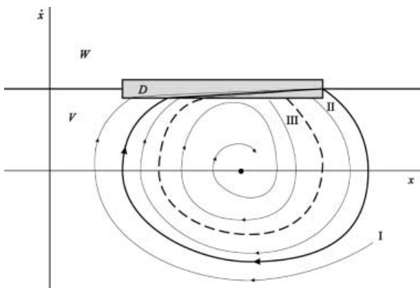
Fig. 6. Phase plane
