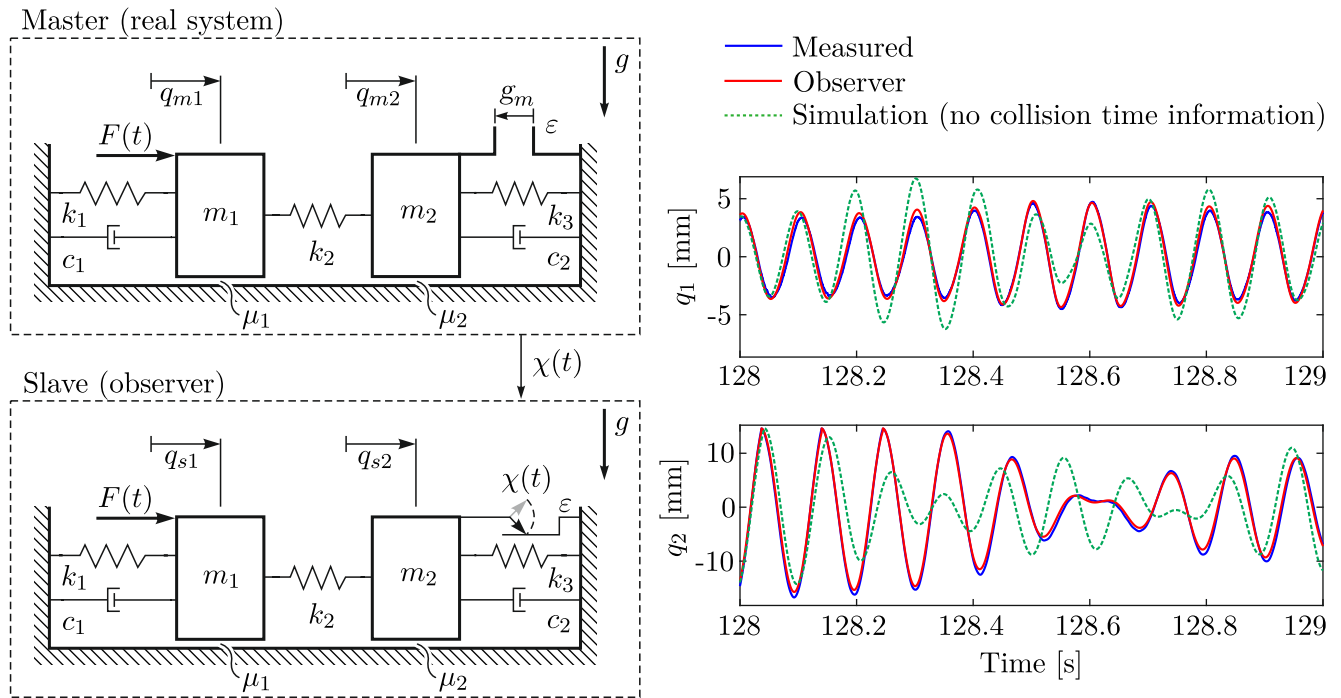
Figure 2: Left: Model of the experimental setup in a master-slave setting. Right: Extract from the time evolution of the measured positions, the observer output and a simulation that only uses the measured excitation force as input.
