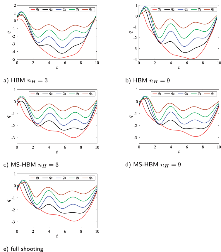
Fig. 5. Displacements of a five DOF oscillator with impact calculated with the different methods
