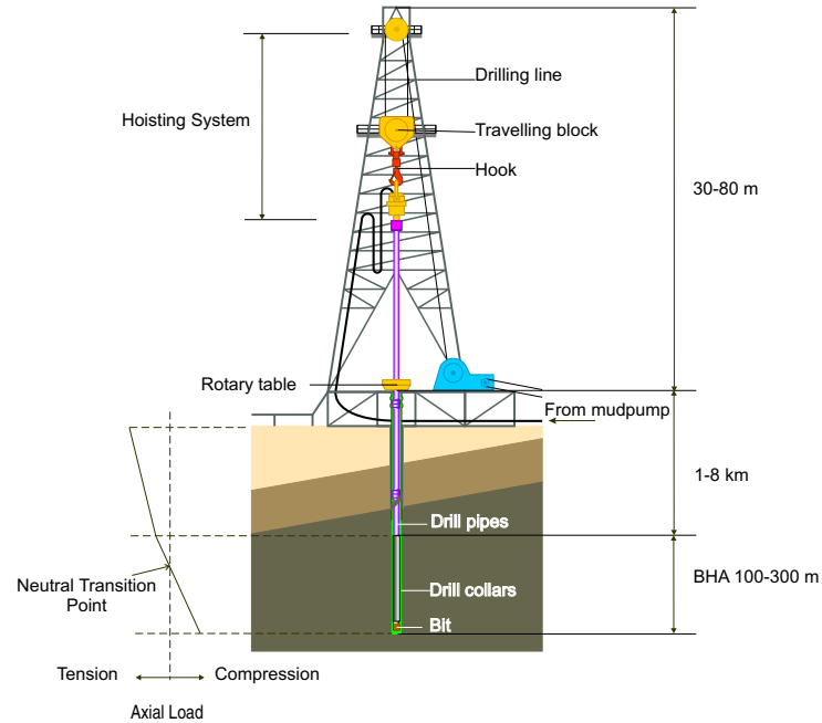
Figure 1. Drilling Rig.
