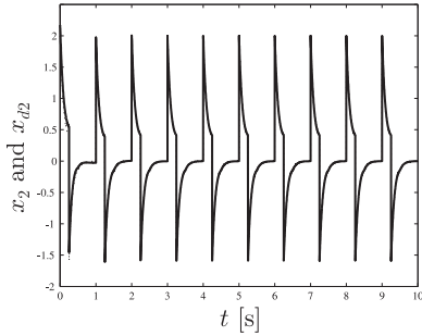
Fig. 5: x_2(t) (solid) and x_{d2}(t) (dotted) for the case of feedback and feedforward control.
