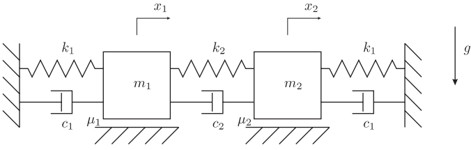
Figure 1: 2DOF mass-spring-damper system with Coulomb friction.
