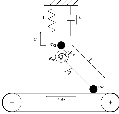
Figure 4.1: The Frictional Impact Oscillator.
